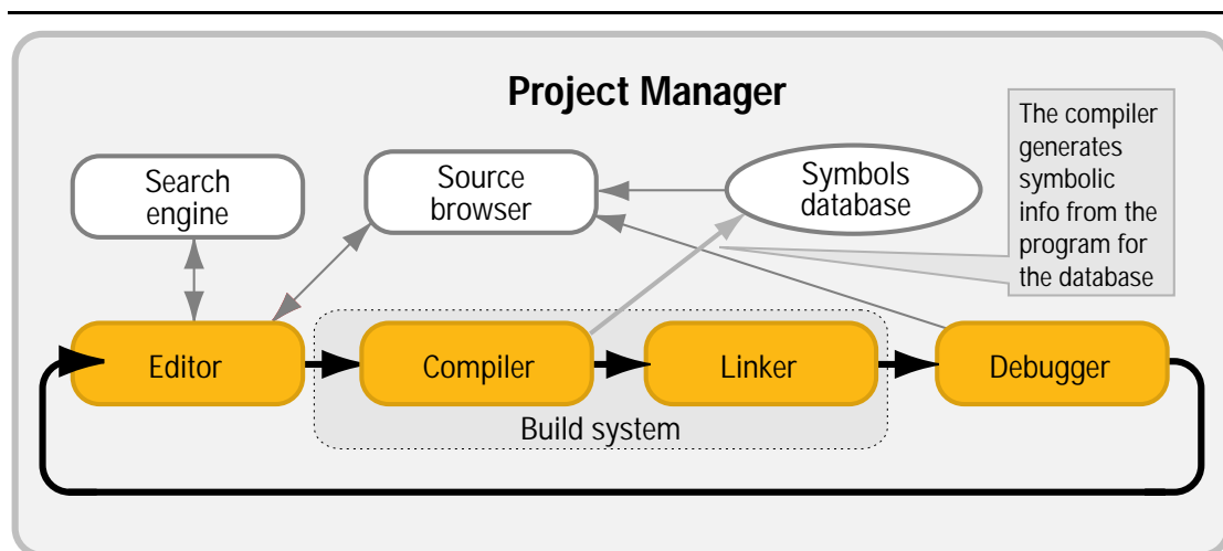
Figure 2: The IDE Architecture
